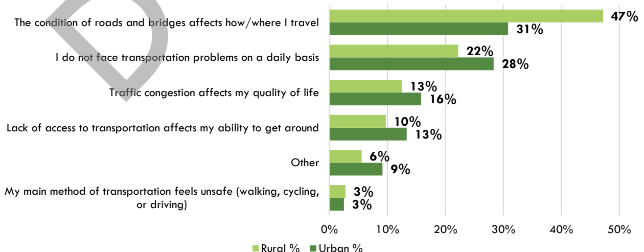
Figure 9: Transportation Problems
